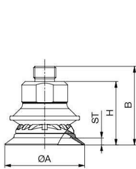
[ EB1.5 / 20 & 40 series ]
