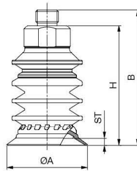
[ EB5.0 / 20 & 40 series ]
