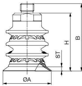
[ B4.0 / 20 & 40 & 60 series ]
