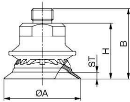
[ B1.5 / 20 & 40 & 60 series ]
